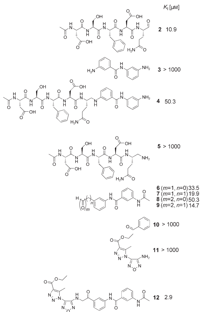
Scheme 1. Development of a non-peptidic SARS-CoV M pro inhibitor through dynamic ligation screening. Active fragment 3 , which binds to the S1' site of the protein, has been transformed into electrophilic derivatives 6–9 , which were employed iteratively in reverted DLS, yielding the non-peptidic inhibitor 12 .
